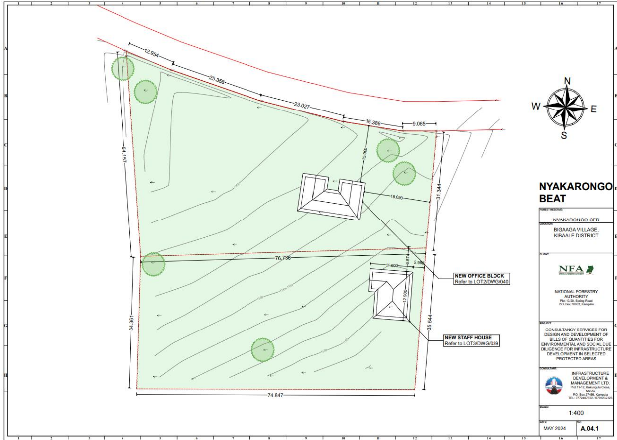
Figure 7: Nyakarongo Site layout Plan
